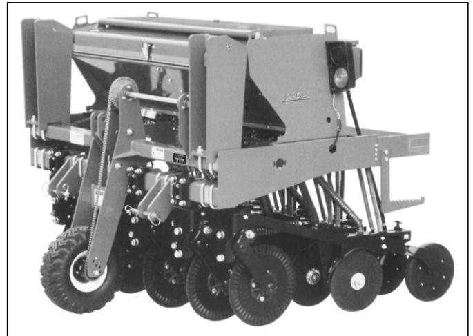
Figure 1 3P606NT No-Till Drill
