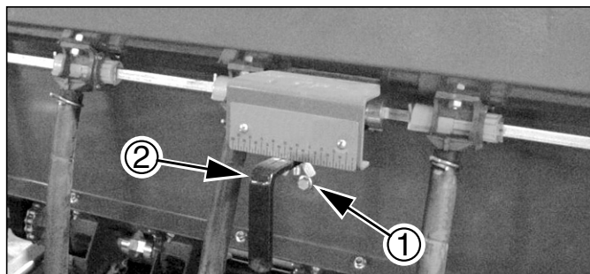
Figure 9 Small Seeds Rate Handle
