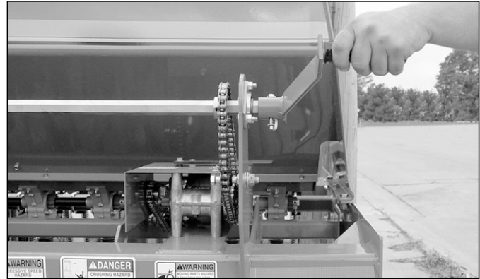
Figure 19 3P606NT Calibration Crank
